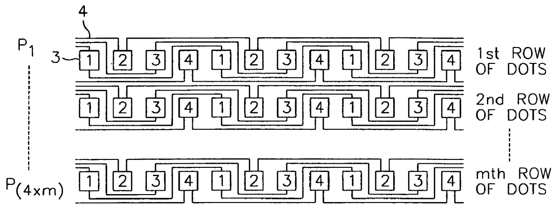
FIG. 8 (PRIOR ART)
